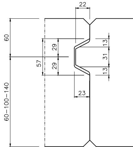
MALE - FEMALE JOINT
